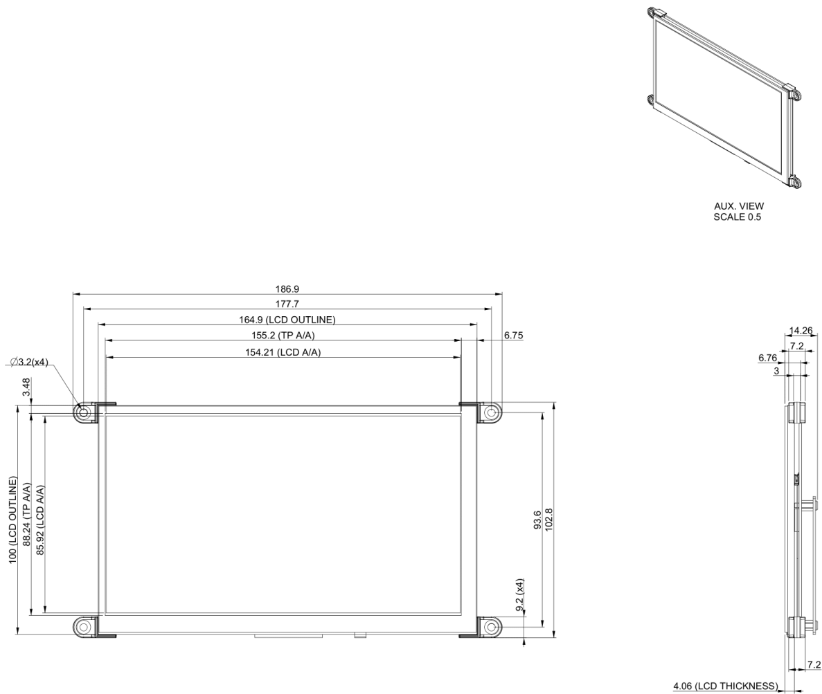
7.0 LCD RTP070
